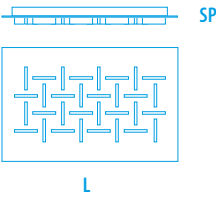
2051/PL 80 W 70 - Vac 230 Lm 5.200 L 500 x 800 mm SP 70 mm
