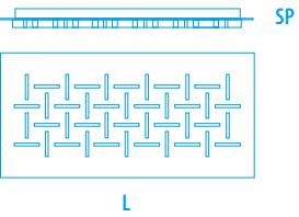
2051/PL110 W 105 - Vac 230 Lm 7.800 L 500 x 1100 mm SP 70 mm
